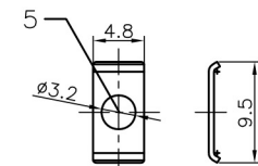
SMALL WASHER
