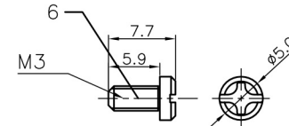
SHORT SCREW
