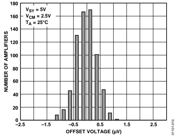
Figure 10. Input Offset Voltage Distribution at 5 V
