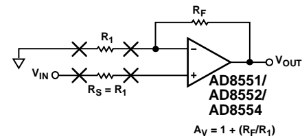
NOTES 1. R_S SHOULD BE PLACED IN CLOSE PROXIMITY AND ALIGNMENT TO R_1 TO BALANCE SEEBECK VOLTAGES.
