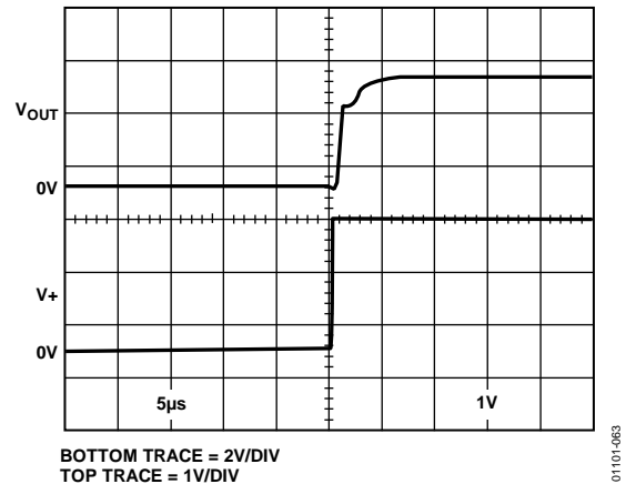
Figure 63. AD8551/AD8552/AD8554 Output Behavior on Power-Up
