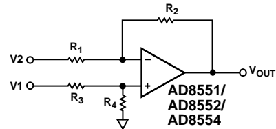
Figure 66. Using the AD8551/AD8552/AD8554 as a Difference Amplifier
