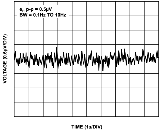
Figure 50. AD8628 Peak-to-Peak Noise
