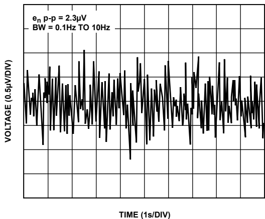
Figure 51. Competitor A Peak-to-Peak Noise
