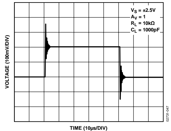
Figure 50. AD8606 Capacitive Load Drive Without Snubber
