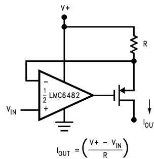
Figure 26. Large Compliance Range Current Source
