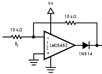
Figure 24. Full Wave Rectifier with Input Current Protection ( R_1 )
