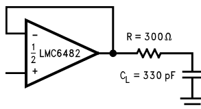
Figure 7. Resistive Isolation of a 330pF Capacitive Load
