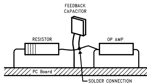
Figure 16. Air Wiring
