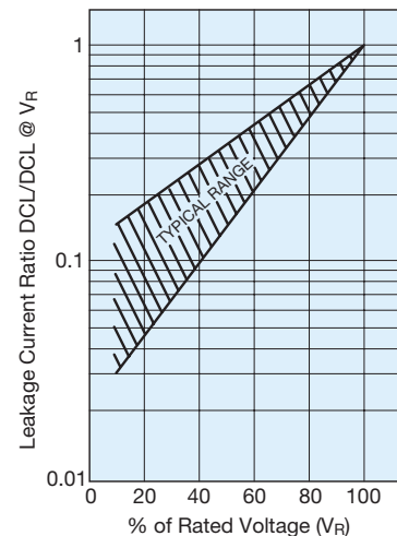
Effect of Voltage Derating on Leakage Current
