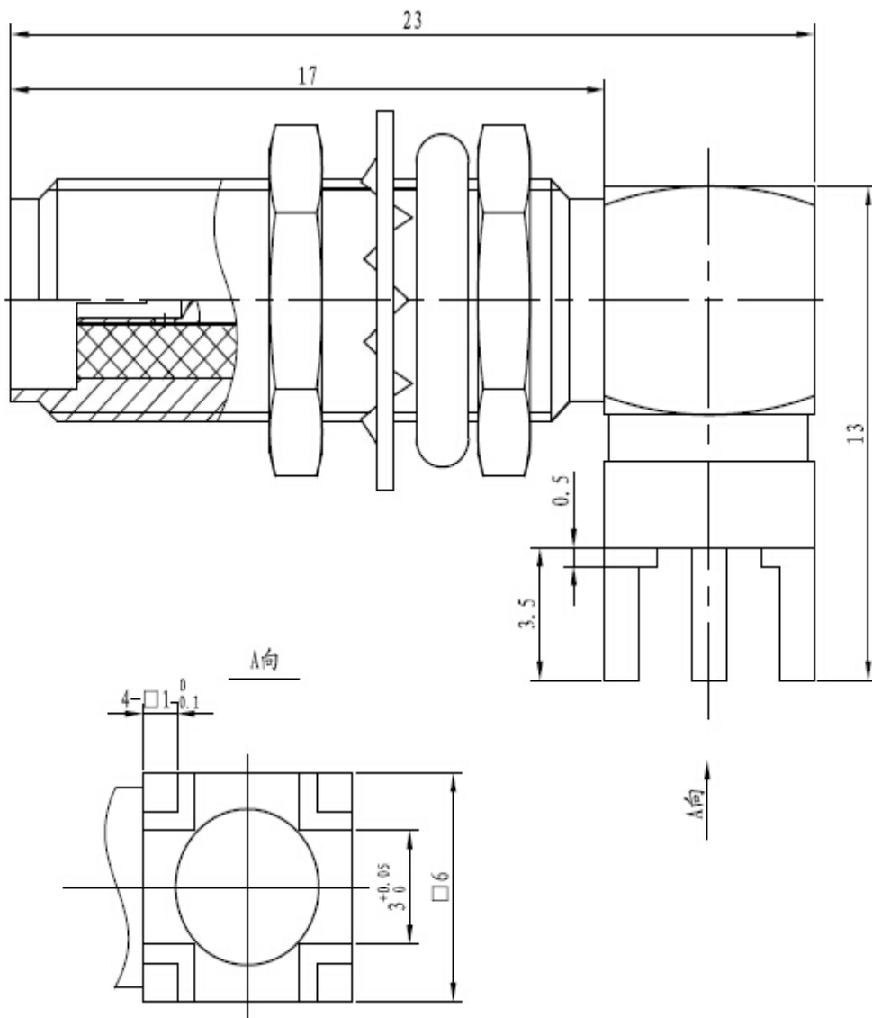
SMA-RWF23
