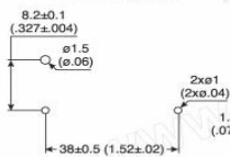
PCB/Mounting Layout
